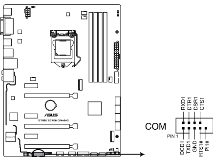
STRIX Z270H GAMING Serial port connector
