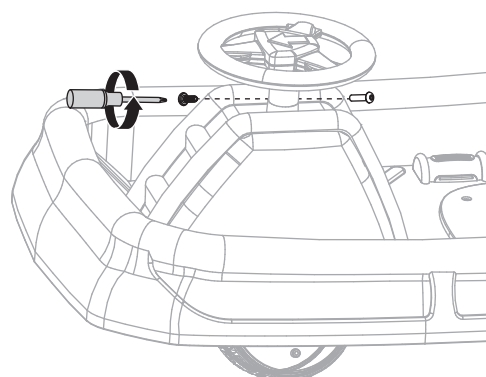
4. Align the holes on the steering wheel with the holes on the front wheel assembly. Re-insert the bolt and tighten securely in place.
