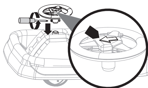
3. Carefully turn unit over. Remove bolt from steering wheel then insert the steering wheel onto the front wheel assembly. Make sure the arrow on the steering wheel is pointing to the front.
