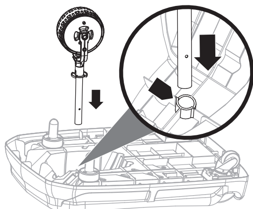
1. Insert front wheel assembly. Note: See Illustrations to the right.
