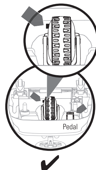
2. Plug the white connector on the front wheel into the white connector on the control module.
