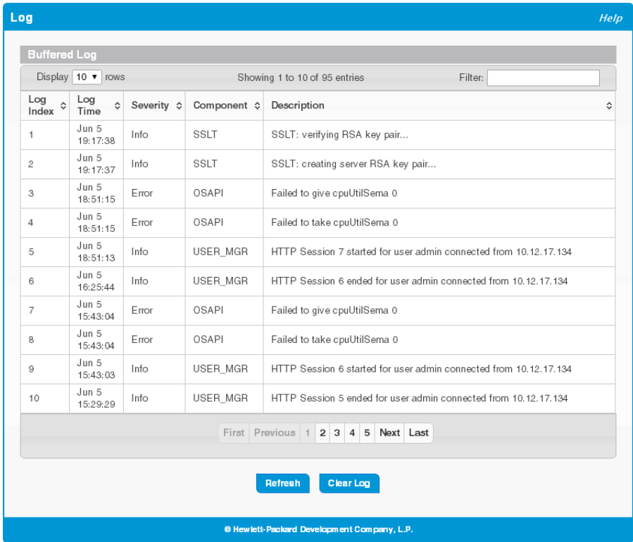
Figure 11-1.Bufferred Log Page
