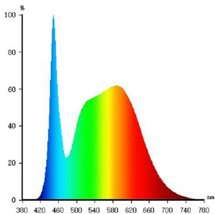
Spectral power distribution(5000K)
