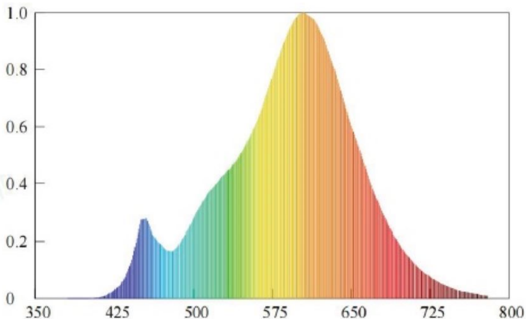
Spectral power distribution(2700k)
