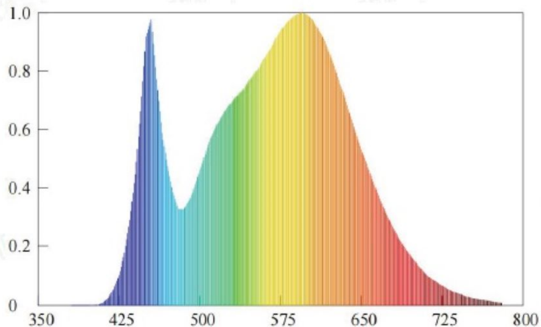
Spectral power distribution(4000k)
