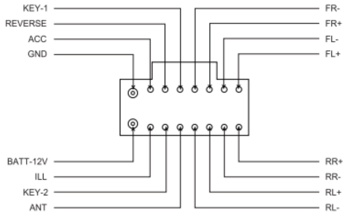
[1] Power Cable Diagram
