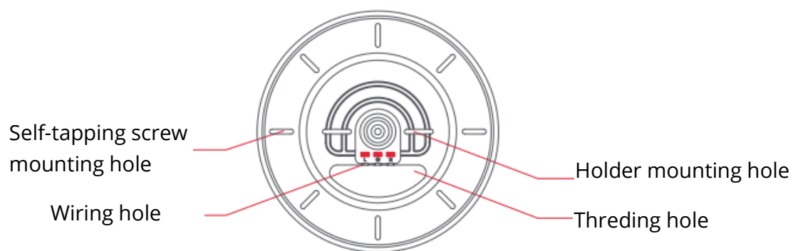
Base plate
