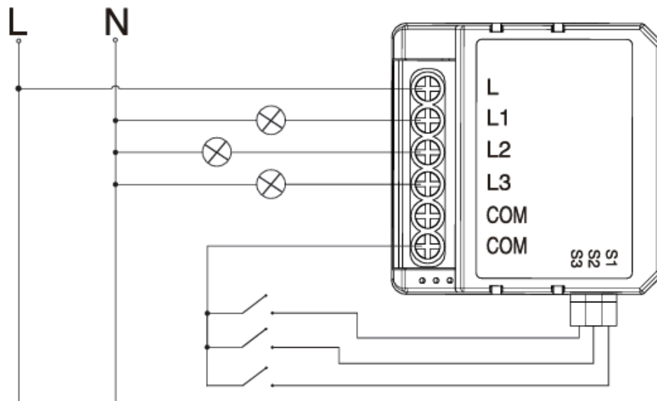
Wiring diagram of fittings (L1 L2 L3 One of them)
