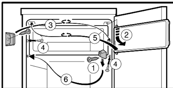
Fig. 6 On appliances with a freezer compartment
