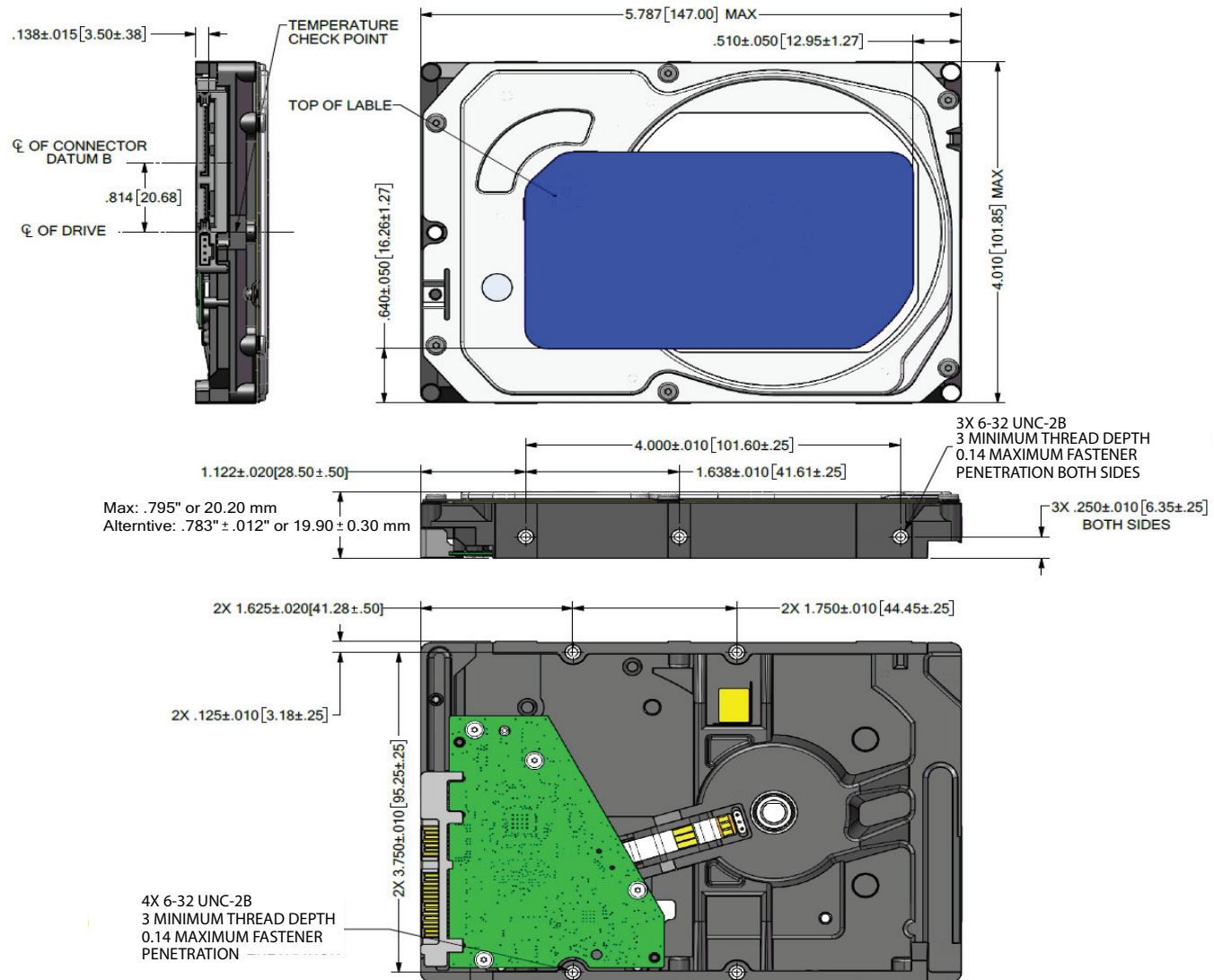
Figure 3 Mounting dimensions (1-disk models)
